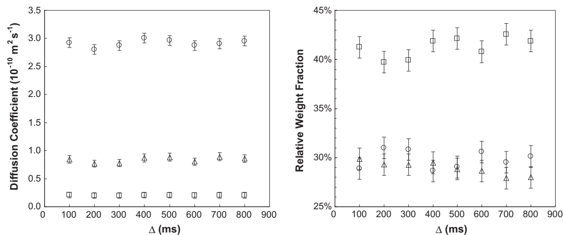
Fig. 4. Diffusion coefficients (left panel) and relative weight fractions (right panel) of PS A ( \circ ), PS B ( \triangle ) and PS D ( \square ) in mixture 4 (A/B/D 30/29/41) as a function of the diffusion delay \Delta . These values were obtained from the signal (7.25–6.89 ppm) associated to the para and meta protons of the phenyl ring.
