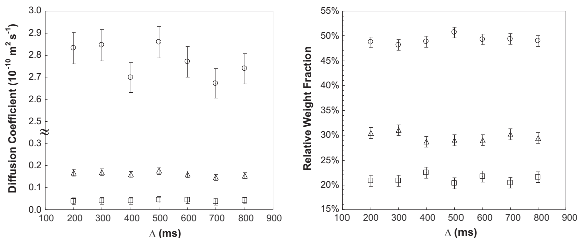
Fig. 3. Diffusion coefficients (left panel) and relative weight fractions (right panel) of PS A ( \circ ), PS C ( \triangle ) and PS E ( \square ) in mixture 3 (A/C/E 46/30/24) as a function of the diffusion delay \Delta . These values were obtained from the signal (7.25–6.89 ppm) associated to the para and meta protons of the phenyl ring.
