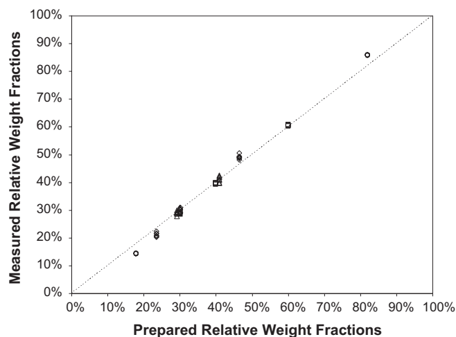
Fig. 5. Relative weight fractions, determined by PGSE NMR, as a function of the prepared relative weight fractions for mixtures 1 ( \square ), 2 ( \circ ), 3 ( \diamond ) and 4 ( \triangle ). These values were obtained from the signal (7.25–6.89 ppm) associated to the para and meta protons of the phenyl ring. The dotted line represents the identity (measured relative weight fractions = prepared relative weight fraction).
